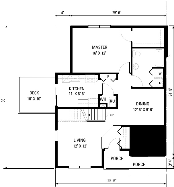
FIRST FLOOR PLAN DOWNHILL CONDITION
