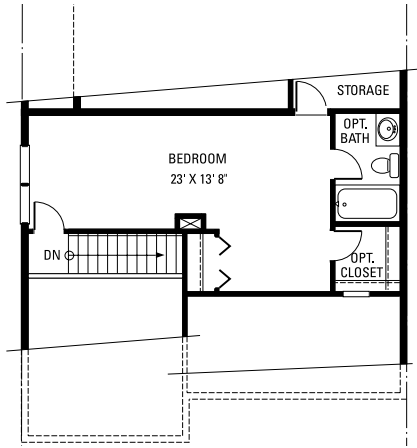
THIRD FLOOR PLAN UPHILL CONDITION SECOND FLOOR PLAN DOWNHILL CONDITION
