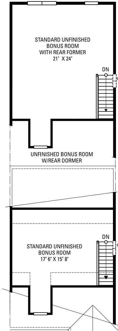
STANDARD UNFINISHED BONUS ROOM
