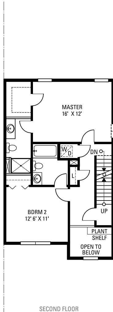
SECOND FLOOR
