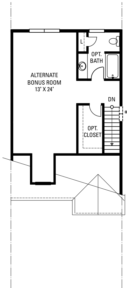
OPTIONAL FINISHED BONUS ROOM WITH REAR DORMER WITH OPTIONAL BATHROOM AND OPTIONAL CLOSET
