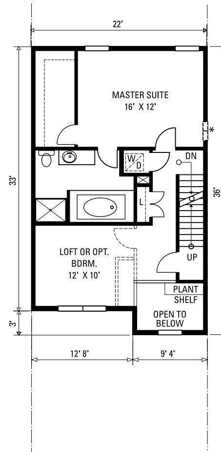
SECOND FLOOR PLAN WITH MASTER SUITE OPTION
